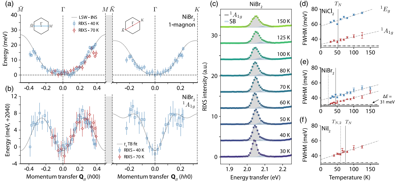
FIG. 4. Momentum dependence of the single magnon (a) and the ^1A_{1g} excitation (b) in \text{NiBr}_2 along the \Gamma M (left) and \Gamma K (right) momentum-space cuts. Blue squares T = 40 K and red diamonds T = 70 K. Experimental single-magnon energies are compared to linear spin wave (LSW) theory, accounting for intralayer exchange up to third nearest neighbor ( J_3 ) using experimentally determined parameters from Ref. [32]. The ^1A_{1g} data are fit along both \Gamma M and \Gamma K with a tight-binding (TB) model considering only third-nearest-neighbor hopping ( t_3 ). The LSW and TB curves are shown as solid gray lines in (a) and (b), respectively. (c) Representative temperature dependence of the ^1A_{1g} excitation in \text{NiBr}_2 highlighting the temperature-dependent linewidth. Gaussian fits to the ^1A_{1g} and its side band (SB) (see text) are the filled gray and blue curves, respectively. Temperature-dependent linewidth of the ^1A_{1g} (red) and ^1E_g (blue) peaks for (d) \text{NiCl}_2 , (e) \text{NiBr}_2 , and (f) \text{NiI}_2 . Linear fits (dashed lines) highlight a linear broadening of each peak with increasing temperature. Horizontal dashed lines denote the experimental resolution ( \Delta E = 31 meV) for all measurements. Vertical solid lines indicate the C-type AFM transition temperature T_N \approx 52, 45 , and 75 K for Cl, Br, and I, respectively, and dashed lines indicate the noncollinear magnetic phases T_{N,2} \approx 22 and 60 K for Br and I, respectively [16,31,64].
