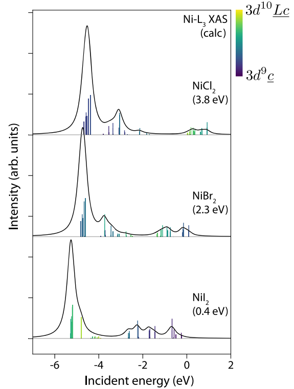
FIG. 7. Calculated Ni- L_3 edge XAS for optimized values in the CTM model for NiCl 2 , NiBr 2 , NiI 2 from top to bottom, respectively. The energy axis is with respect to the center energy of the 3d^9 2p^5 configuration in the calculation. Individual excitations contributing to the XAS profile are shown as bar plots over the corresponding spectra, showing the evolution of each XAS transition between the 3d^9 \underline{c}/3d^{10} \underline{Lc} ligand-hole character as \Delta is reduced. The relative weight of each configuration is indicated by the color bar. See also the analogous plot for the ground-state multiplets in Fig. 2(b).
